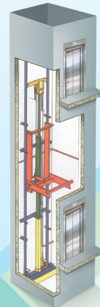
Indirect Side Acting 2:1
