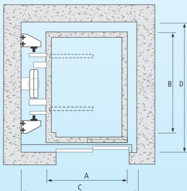
ROPE TYPE - Single Cylinder
