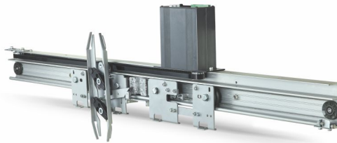
2-Panel Centre Opening Car Door Mechanism
